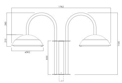
TWIN BRACKET
