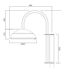
SINGLE BRACKET
